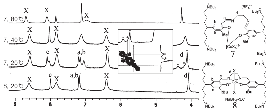
Figure 1. The ^1\text{H} NMR spectra of 7 and 8 in \text{DMSO-d}_6 . The signals marked with “X” are assigned to 2,4-dinitrophenolate. The box shows a selected region of the ^1\text{H} – ^1\text{H} COSY NMR spectrum of 7 at 20 °C.
